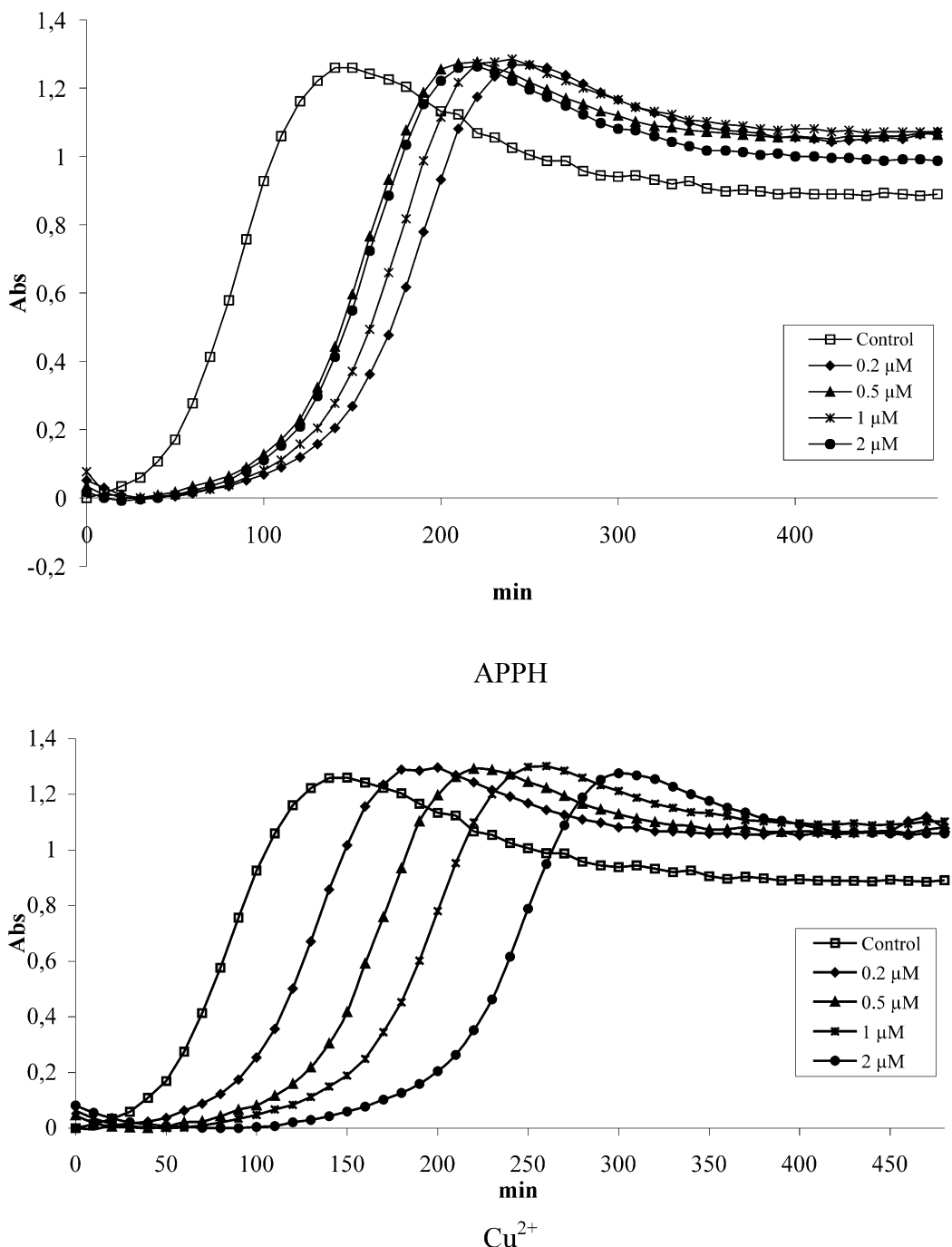
Figure 1. Effect of 1 on the lag phase of LDL oxidation by copper (II) and AAPH by increase of the diene absorption. The LDL solution (125 \mu\text{g} protein/mL) was supplemented with 0, 0.2, 0.5, 1, 2 \mu\text{M} of 1 in 0.01 M PBS. 26 The reference cuvette contained LDL and 1 without copper or AAPH.
