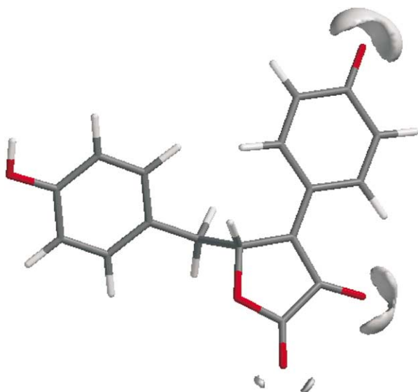
Figure 4. Structure of 1^{\bullet-} .
