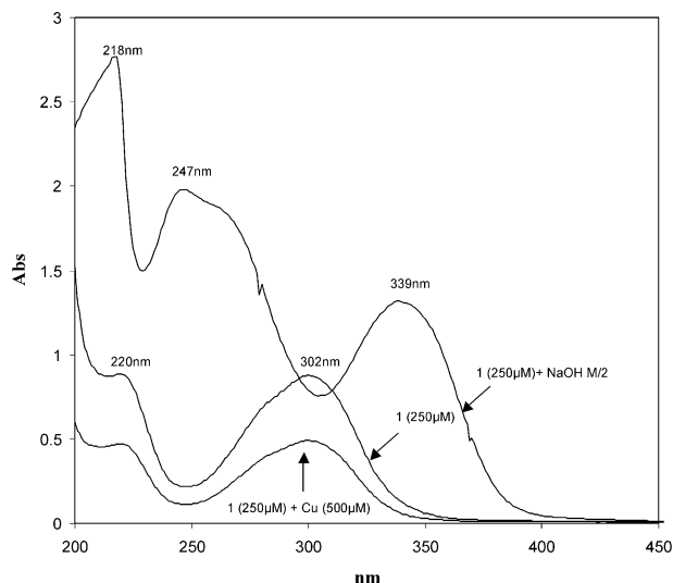
Figure 2. UV spectra of 1 in aqueous solution, after addition of Cu^{2+} or after addition of NaOH M/2.
